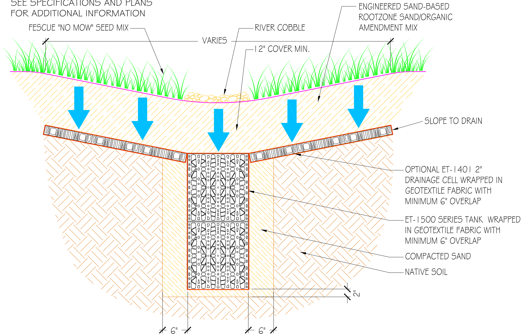
CONCEPT SWALE SECTION WITH 2" CELLS
