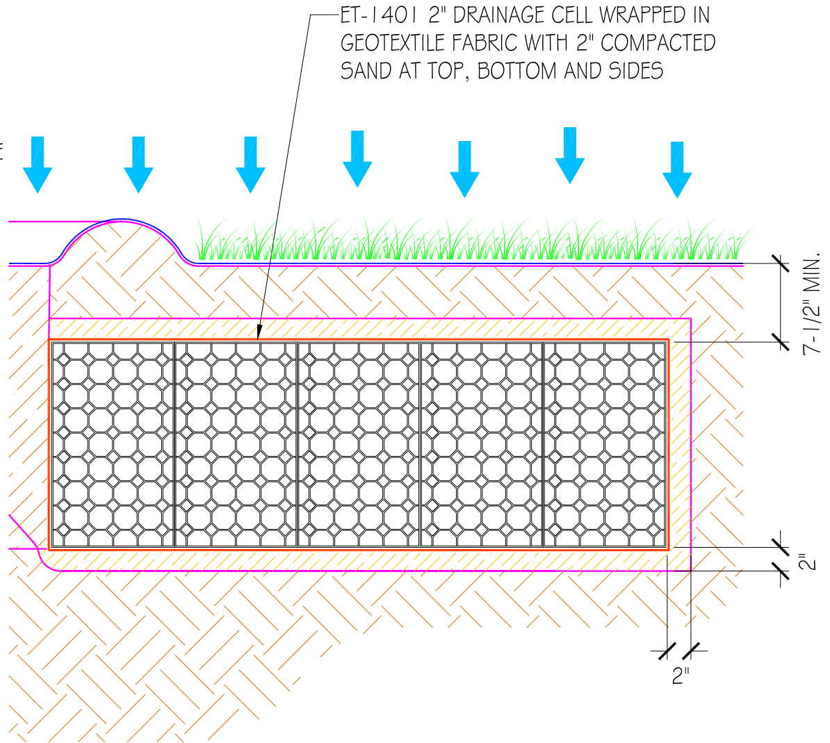
ENLARGEMENT - TYPICAL TREE DETAIL ELEVATION
